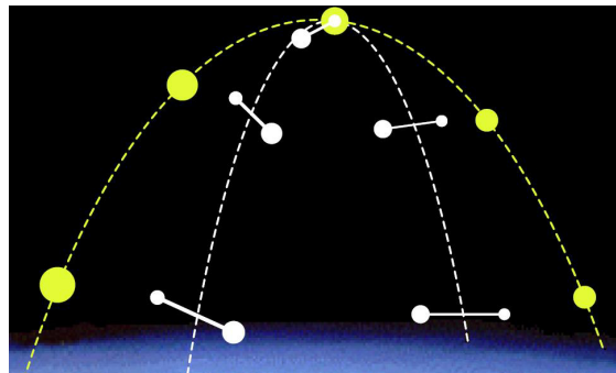
Fig. 5. Rendezvous by EDDE tip in flat spin.
